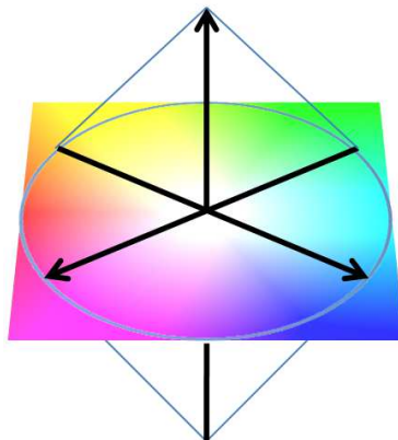
HSV
